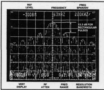
Figure 26. Frequency domain display of pulse waveform.
