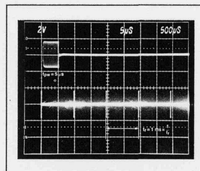
Figure 25. Time domain display of pulse waveform.
