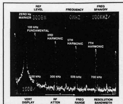
Spectrum Analyzer Waveform: 100 kHz Square Wave
