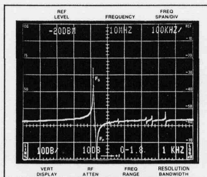
Figure 23. Crystal response to SA/TG system.
