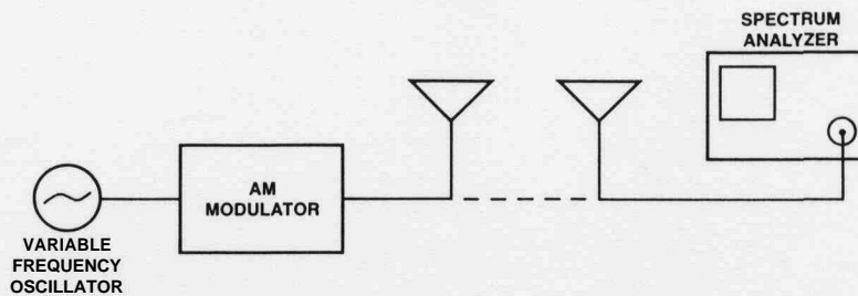
Figure 15. Test setup for sweeping audio flatness.
