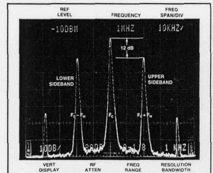
Figure 12. AM Modulation in frequency domain.
