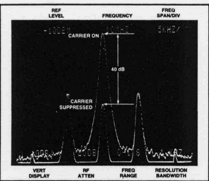
Figure 14. Suppressed Carrier System
