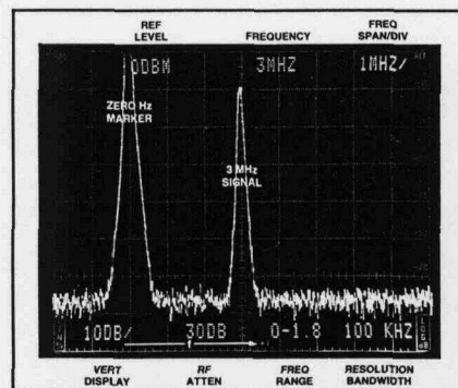
Spectrum Analyzer Waveform: 3 MHz Sine Wave
