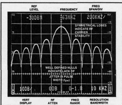
Figure 27. Envelope of pulsed signal
