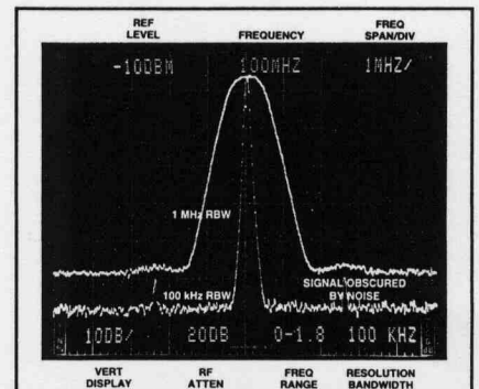
Figure 10. Composite photograph illustrating sidebands obscured by noise in wider resolution bandwidth.
