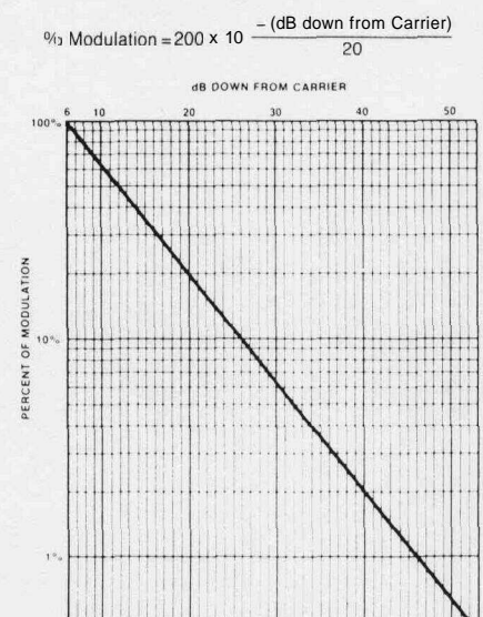
Figure 13. Chart of dB vs. % of Modulation.
