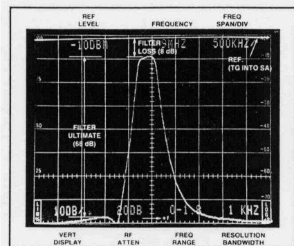
Figure 21. Filter response of filter using SA/TG.
