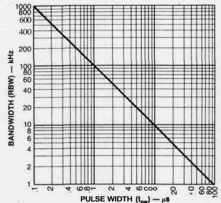
Figure 28. Resolution bandwidth setting for pulsed RF computed from [t_{pw}] \times \text{RBW} = 0.1
