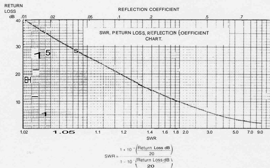
Figure 36. SWR, Return Loss, and Reflection Coefficient Chart.
