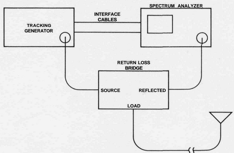
Figure 34. SWR test setup.
