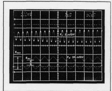
Figure 11. AM Modulation (50%) in time domain.
