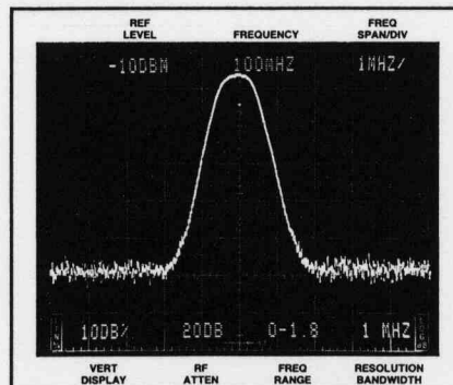
Figure 8. 1 MHz RBW. Wider Than Optimum Bandwidth
