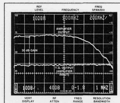
Figure 24. Amplifier response to SA/TG system.
