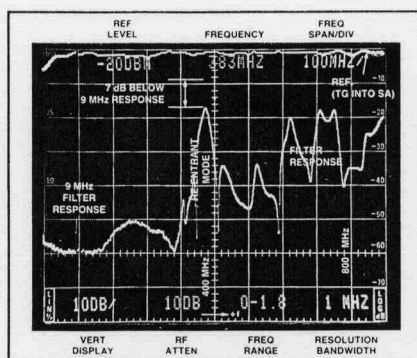
Figure 22. Filter response at wide sweep indicating re-entrant mode.
