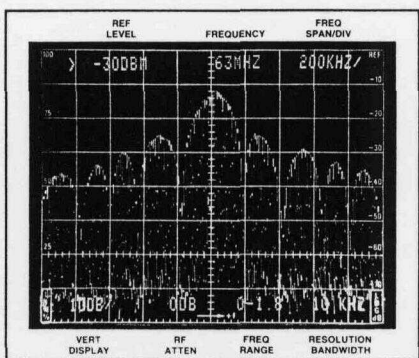
Figure 31. FM'ing carrier.
