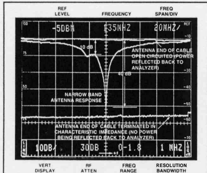
Figure 35 Return Loss of Narrow Band Antenna with 40 dB Return Loss.
