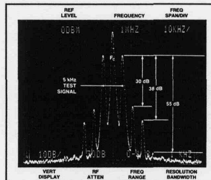
Figure 17. Harmonic Distortion at 10 kHz, 15 kHz, and 20 kHz from Carrier.
