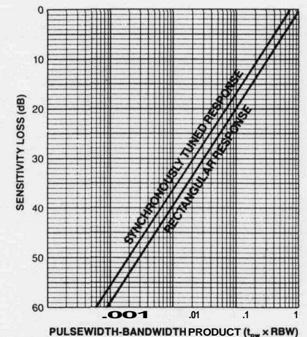
Figure 29. Sensitivity loss of pulsed signals vs CW.
